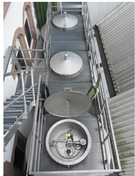
View of a VEGAPULS 63 radar level transmitter on one of the maturation vessels.
