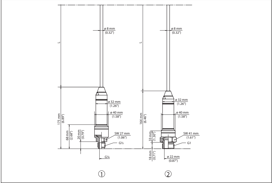
Res. 36: VEGABAR 86, Dişli model
