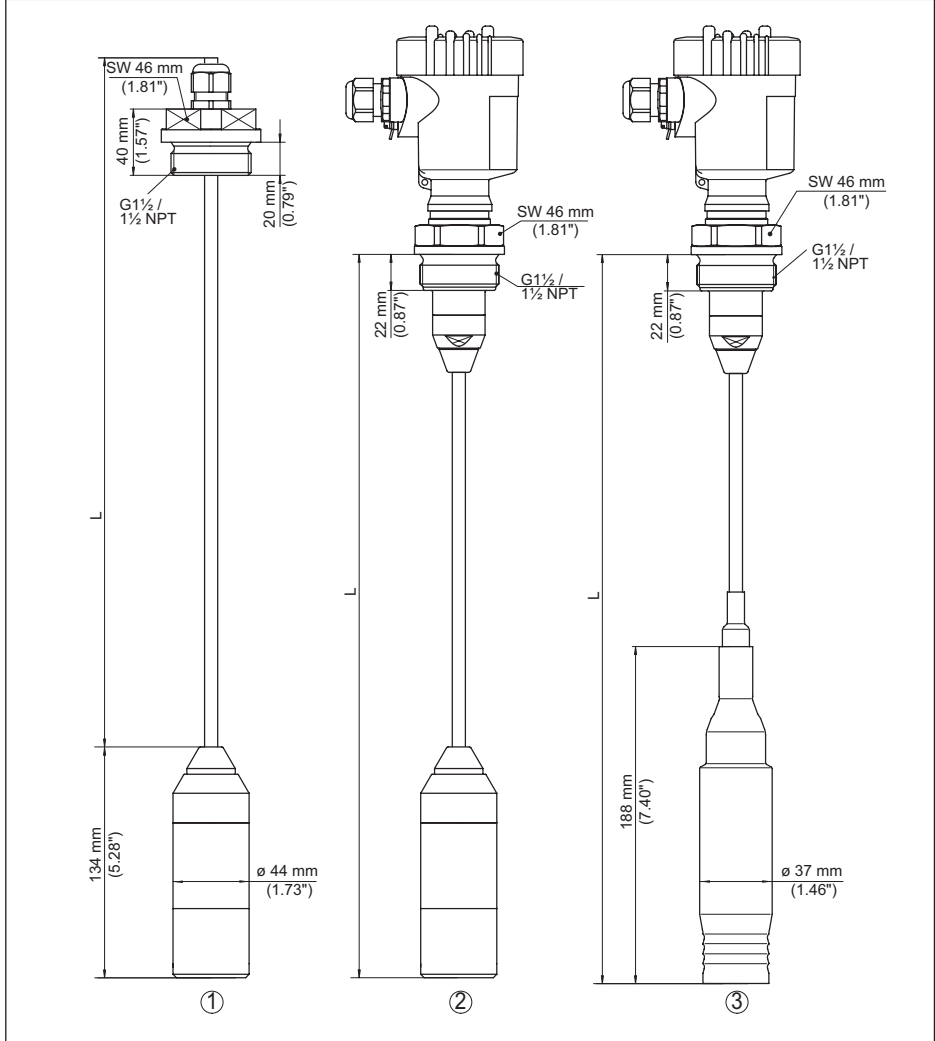
Res. 30: VEGABAR 86, plastik model
