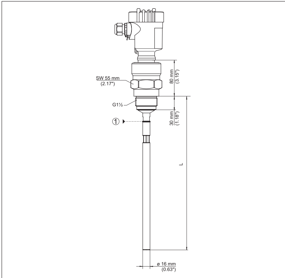
Fig. 51: VEGAFLEX 82, haste \varnothing 16 mm (0.63 in), modelo com rosca
