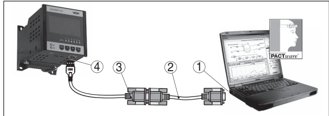
Fig. 11: Raccordement du PC via RS232
