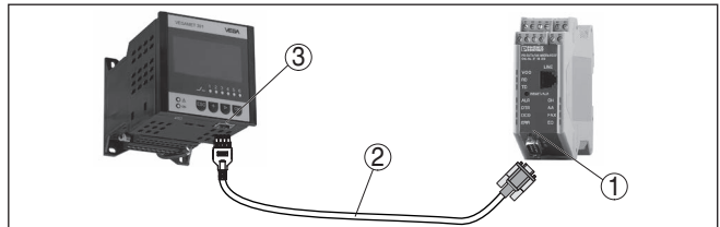
Fig. 10: Raccordement du modem via RS232
