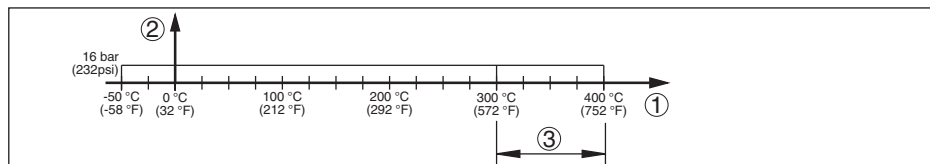
Fig. 20: Température process - pression process
