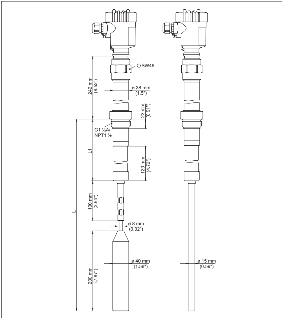
Fig. 23: VEGACAP 67, version fileté G1 1/2" (ISO 228 T1) et 1 1/2" NPT, -50 ... +300 °C (-58 ... +572 °F)
