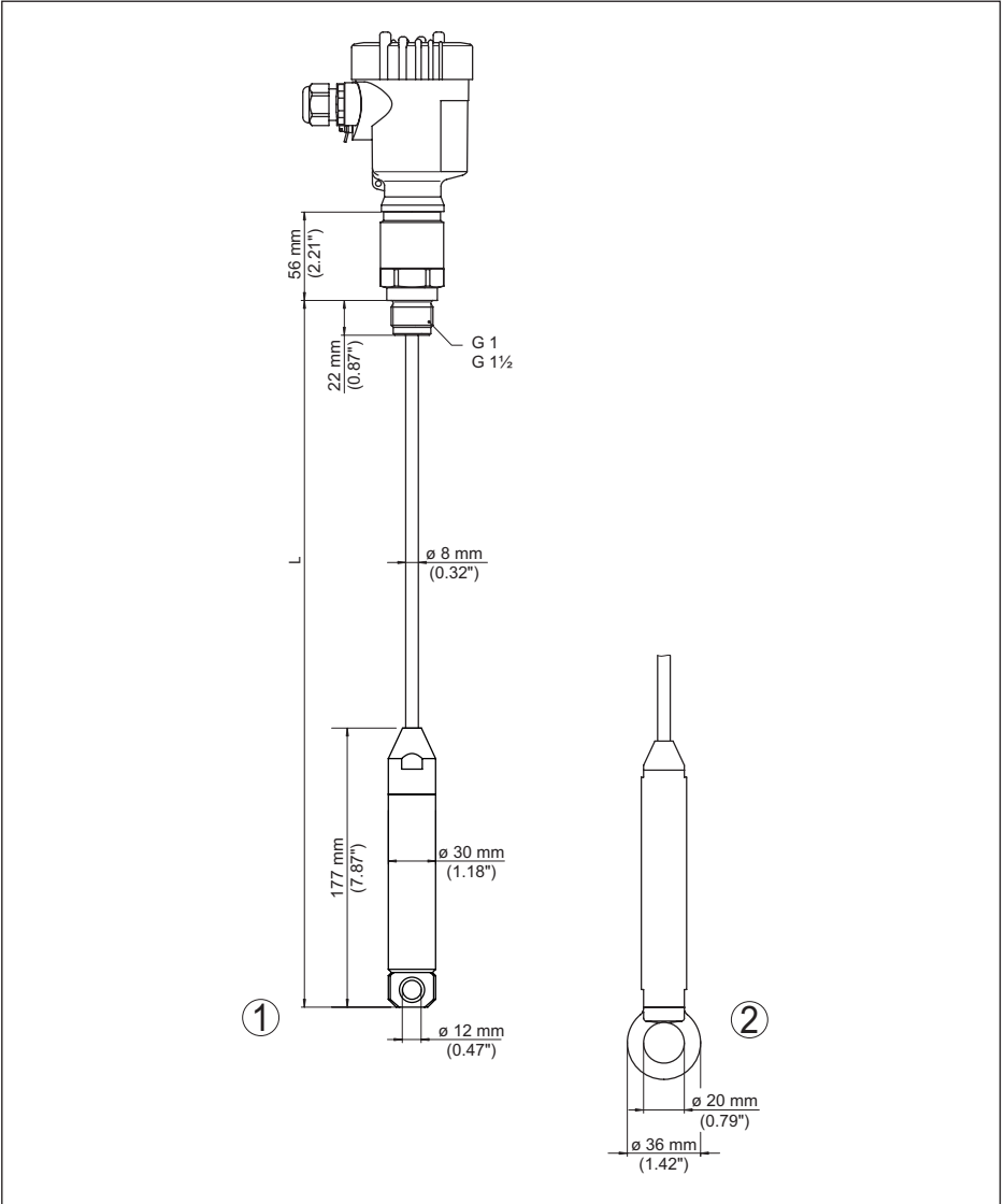
Res. 19: VEGACAL 66, G1 dişli modeli (ISO 228 T1)
