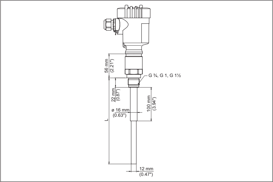
Fig. 19: VEGACAL 62, version fileté G1 (ISO 228 T1)
