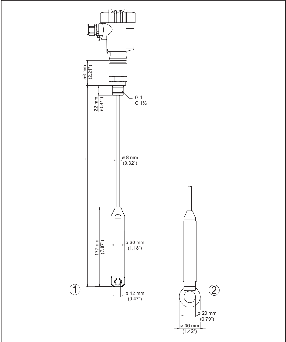
Res. 33: VEGACAL 66, G1 dişli modeli (ISO 228 T1)
