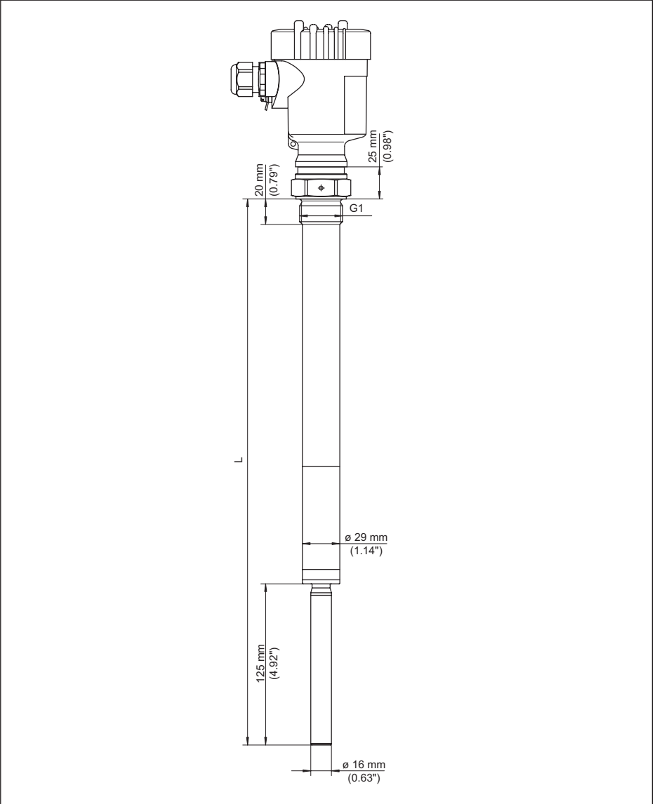
Res. 18: VEGAVIB 63, G1 dişli modeli ((DIN ISO 228/1)
