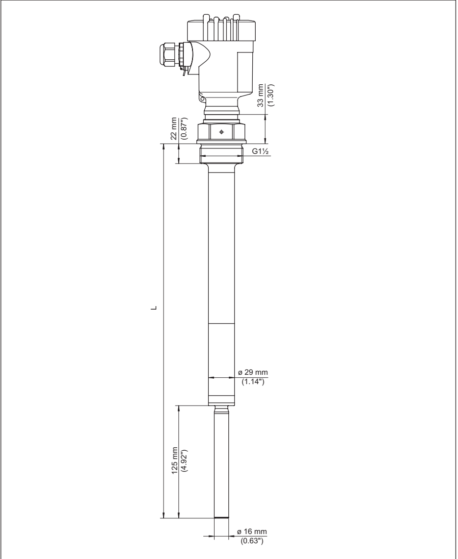
Res. 19: VEGAVIB 63, G1½ dişli modeli (DIN ISO 228/1)
