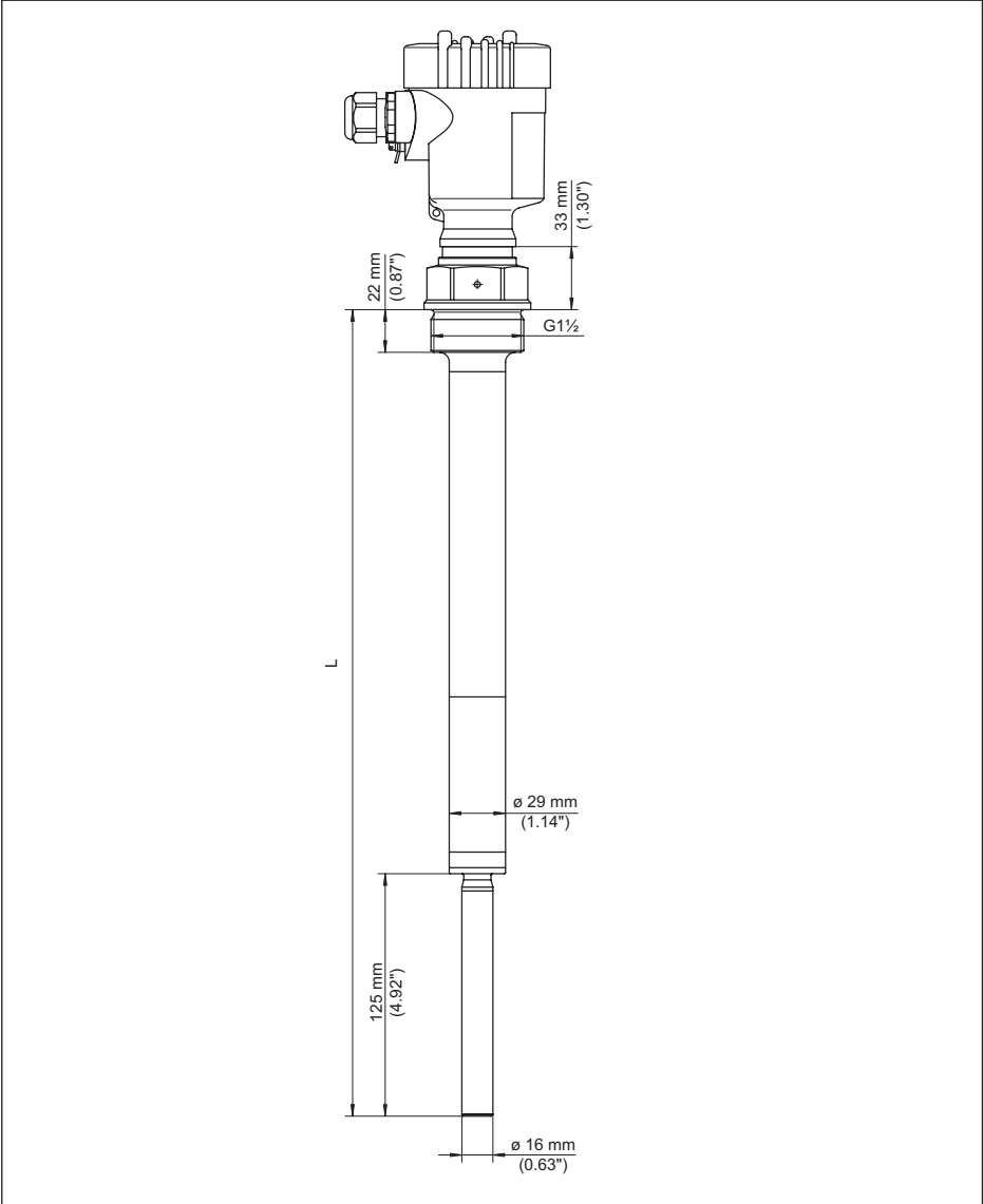
Res. 16: VEGAVIB 63, G1½ dişli modeli (DIN ISO 228/1)
