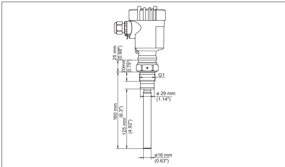
Fig. 20: VEGAVIB 61 - version fileté G1 (DIN ISO 228/1)
