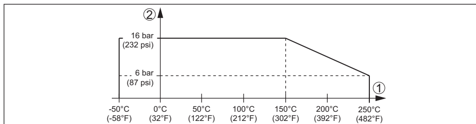
Fig. 16: Pression process - température process
