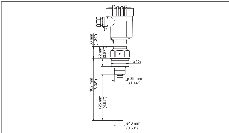
Fig. 21: VEGAVIB 61 - version fileté G1½ (DIN ISO 228/1)
