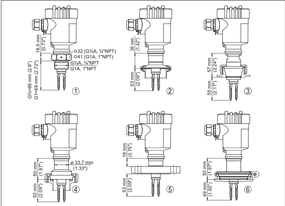
Abb. 21: VEGASWING 61
