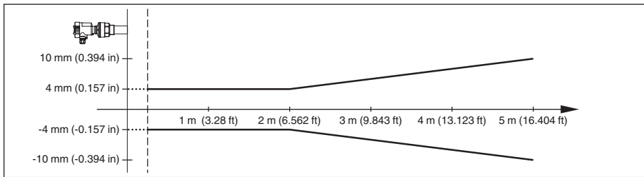
Fig. 35: Meetafwijking VEGASON 61
