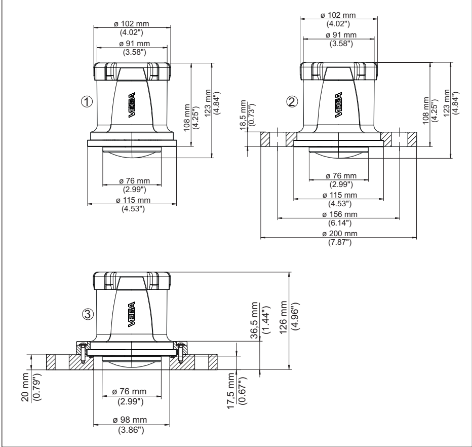
Res. 29: Ebatlar - VEGAPULS Air 42
