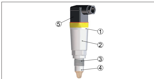
Rys. 1: VEGAPOINT 31
