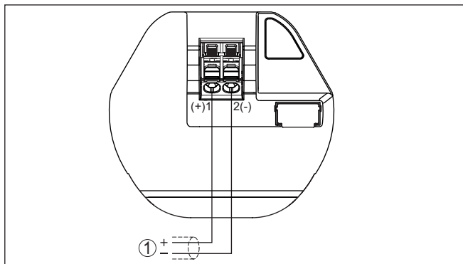
Fig. 19: Compartiment de raccordement VEGAPULS 11
