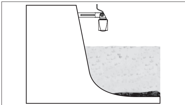
Fig. 15: Peilmeting stuwdam, sensormontage op console
