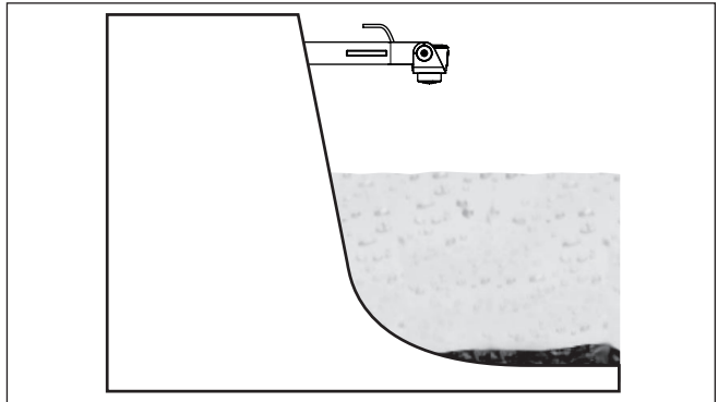
Fig. 16: Peilmeting stuwdam, sensormontage op console
