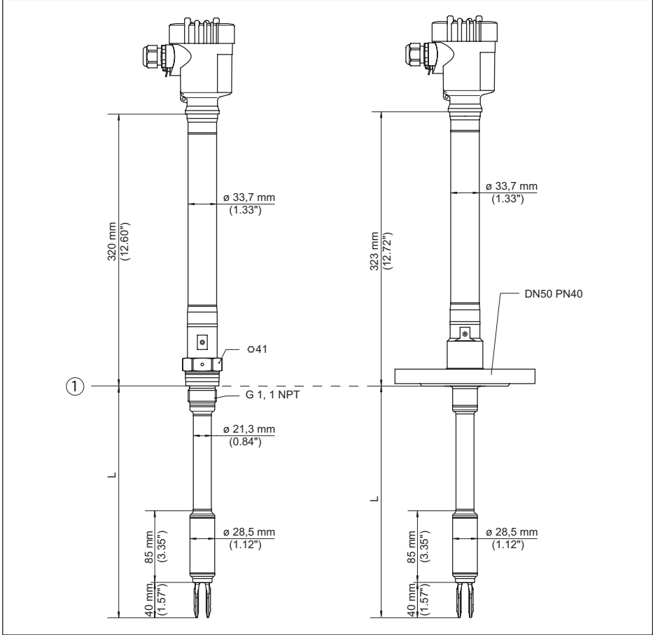
Res. 22: VEGASWING 66, Boru modeli
