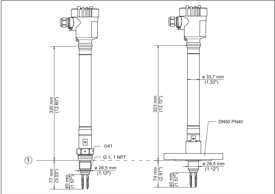
Res. 21: VEGASWING 66, Kompakt model
