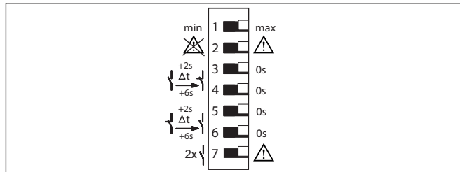
Abb. 2: DIL-Schalter VEGATOR 121
