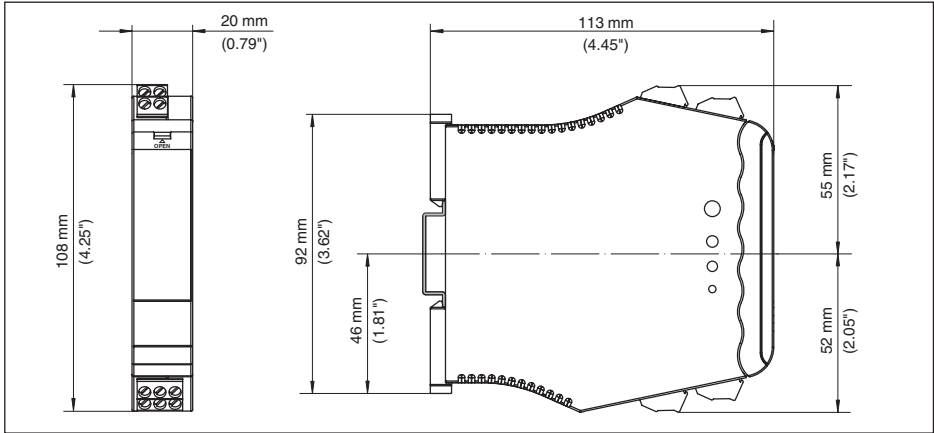
Fig. 2: Dimensions VEGATRENN 152
