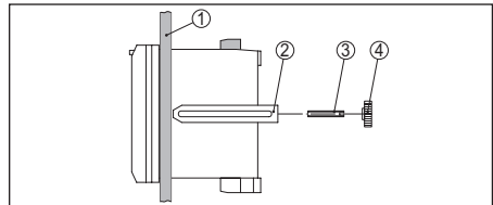
Abb. 11: Front panel mounting
