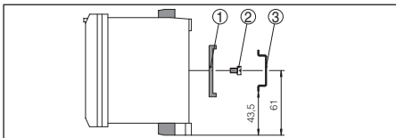
Abb. 13: Carrier rail mounting
