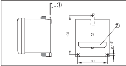
Abb. 12: Screw mounting
