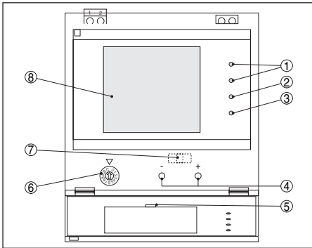
Abb. 16: Display and adjustment elements
