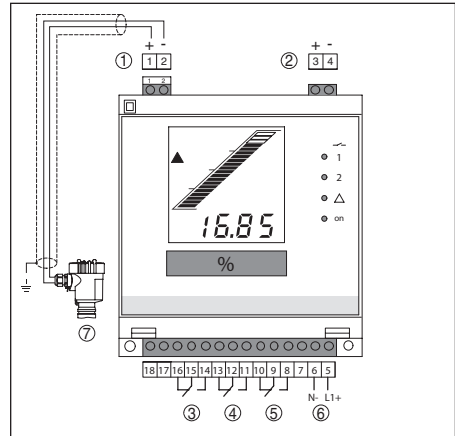
Abb. 15: Wiring plan with two-wire sensor
